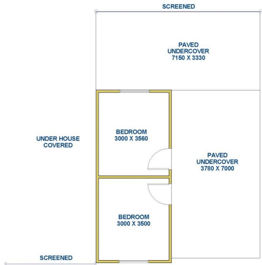
Ground Level
