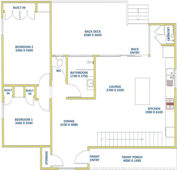
GROUND LEVEL
